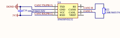
CAN2 Transceiver
