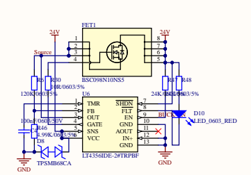
Surge Stopper
